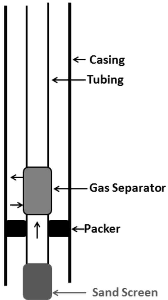
Figure 14 - Packer Type Separator with Sand Screen
