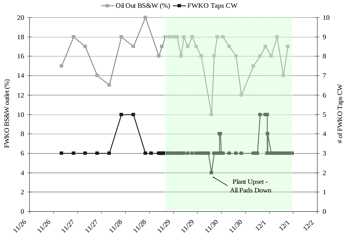
Chart 4 - Oil Outlet BS&W vs. FWKO Taps
