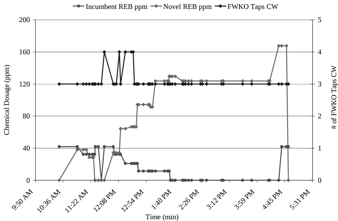
Chart 1 -PPM vs. FWKO Taps of Clean Water
