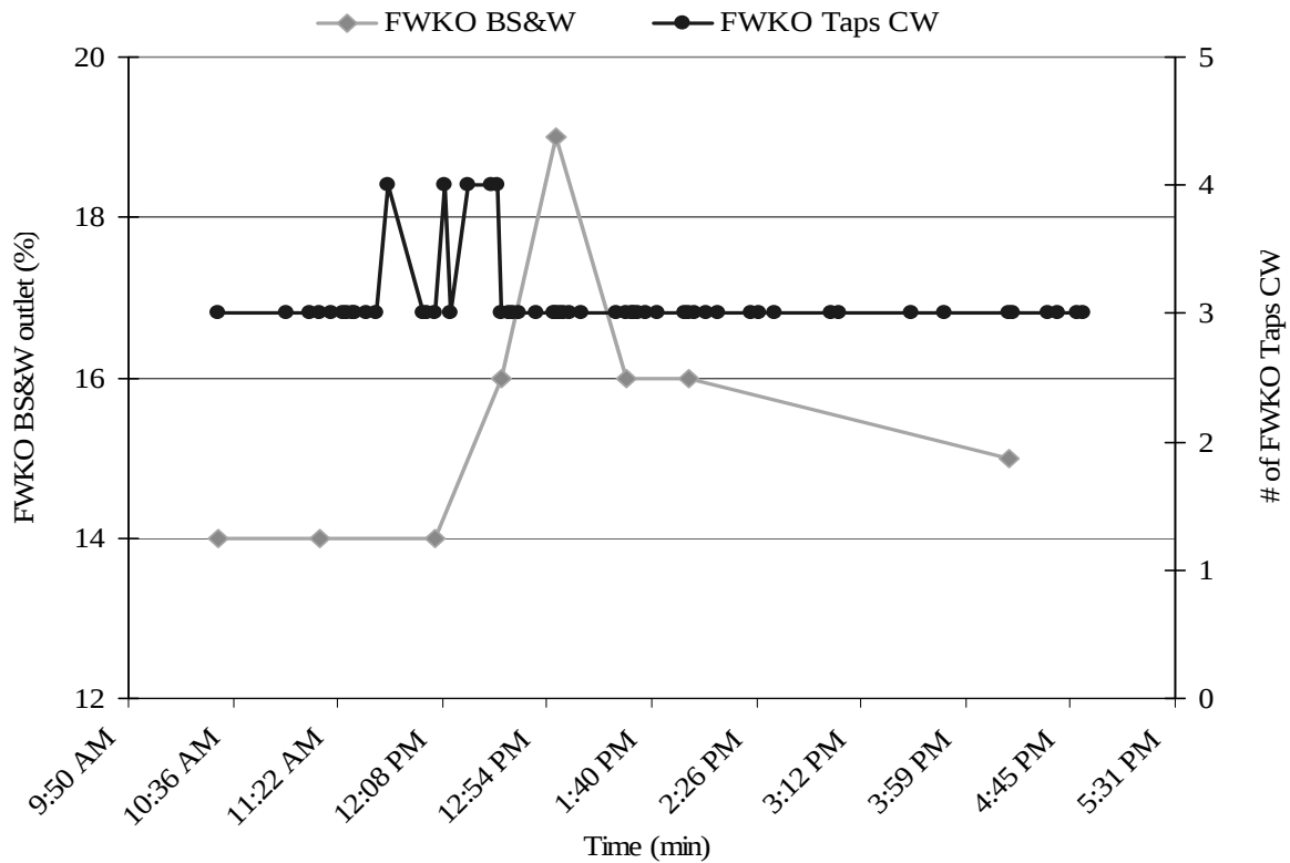
Chart 2 - FWKO Taps vs. Oil Outlet BS&W
