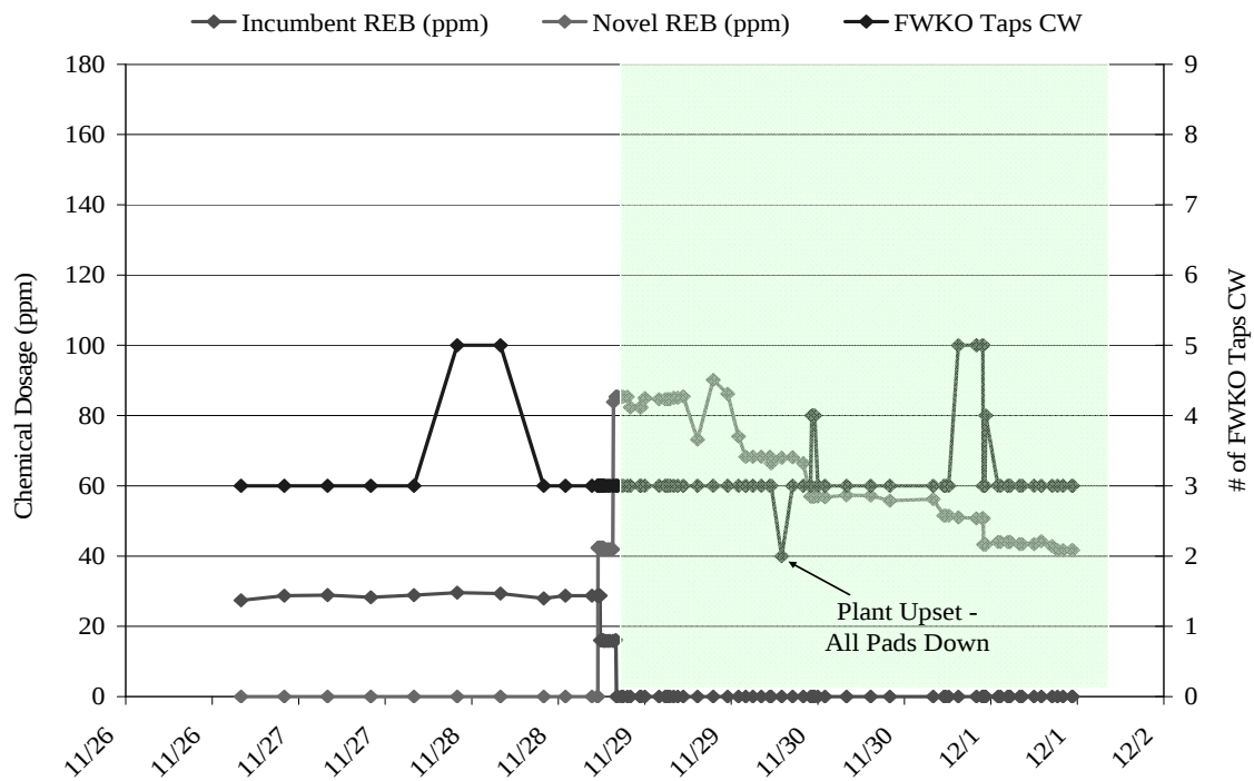
Chart 3 - PPM vs. FWKO Taps of Clean Water
