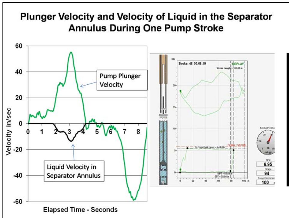
Figure 4 – Pump Plunger Velocity and Velocity of Liquid in Separator Annulus for Conventional Beam Pump Operating at 6.95 Strokes per Minute.
