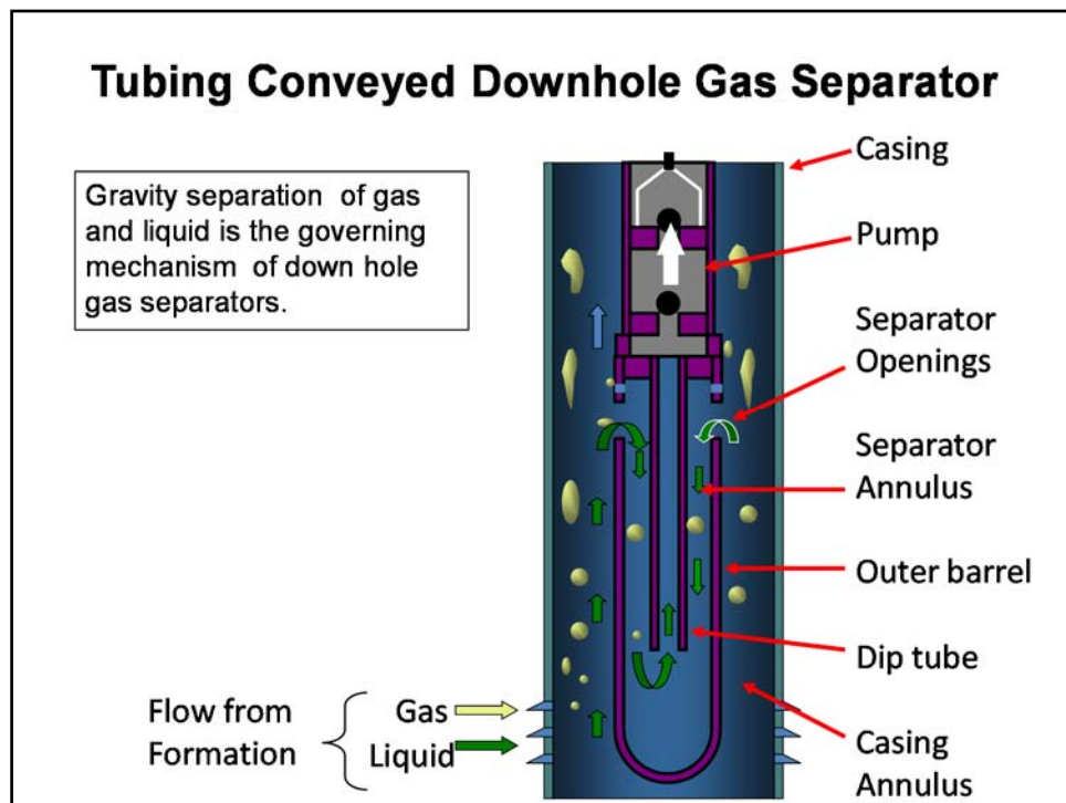
Figure 1 – Schematic Diagram and Definition of Terms for a Tubing Conveyed Down Hole Gas separator 1 .
