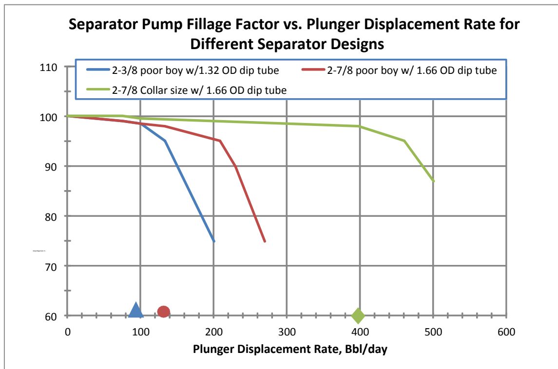
Figure 3 – Pump Fillage Factor as a Function of Plunger Displacement Rate for 3 Separator Designs. (Colored markers on horizontal axis indicate individual separator capacities from Table 1)
