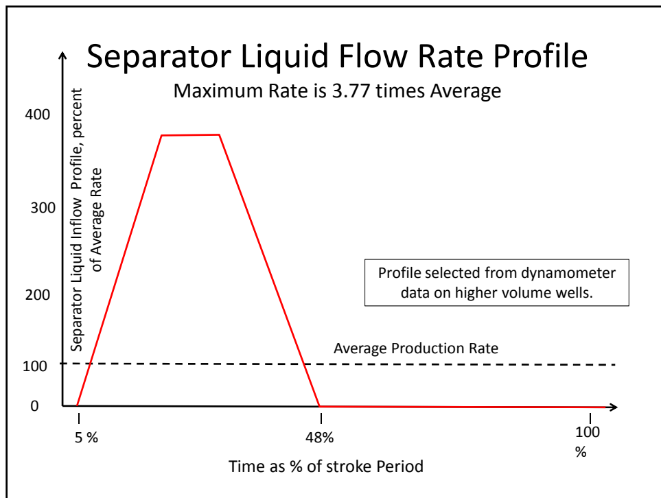
Figure 5 – Generalized Liquid Inflow Profile for Separator Simulation
