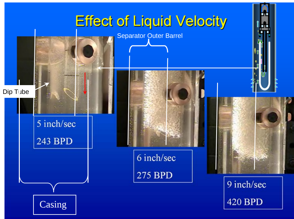
Figure 2 – Video Snap-shots of Gas Bubble Concentration 2 in Separator Annulus as a Function of Downward Liquid Flow Rate for Annular Area of 5.15 in 2
