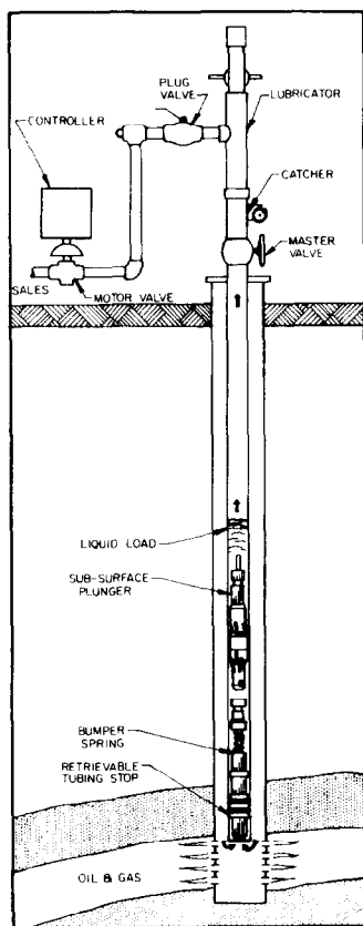
Typical plunger installation. FIG. 1
