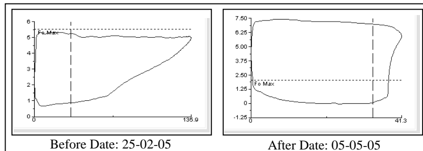
Figure 3 - Dynagraphic Charts Before and After on Well MFA-073
