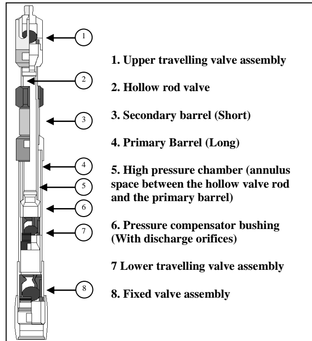
Figure1 - Mechanical Diagram of the Equipment
