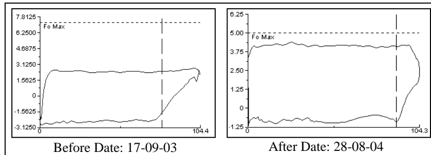
Figure 2 - Dynagraphic Charts Before and After on Well MEL-72
