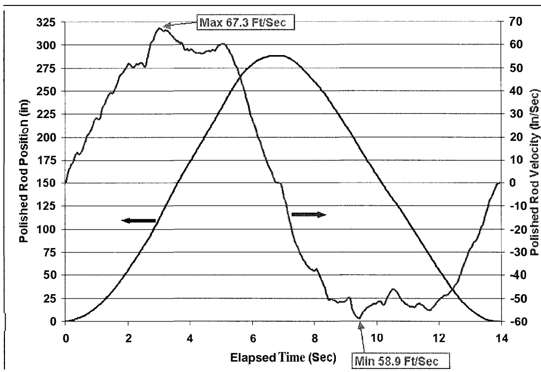
Figure 2 – DynaPump Control of Speed During One Stroke
