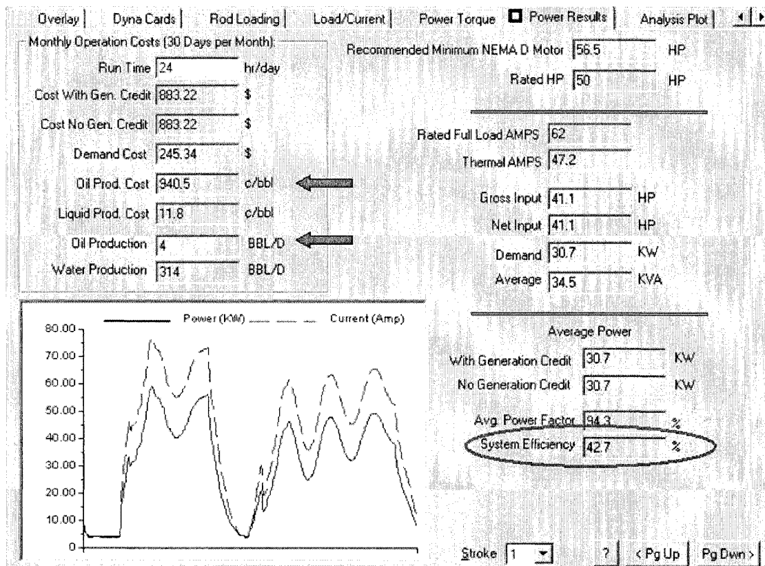
Figure 5 - System Efficiency Analysis, 43% System Efficiency w/ 67 BPD Leakage, 09/12/2002
