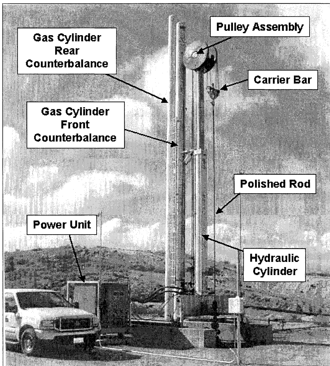
Figure 1 - DynaPump System
