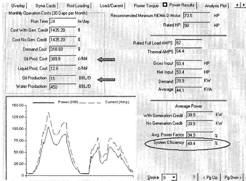
Figure 11 - Highest System Efficiency Analysis, Fastest Rate, 10/22/2002
