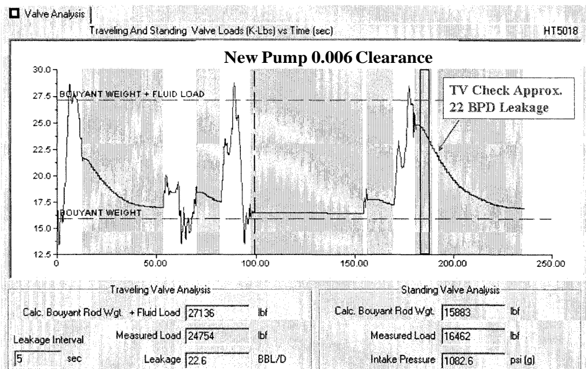
Figure 7 - Dynamometer Analysis, Valve Checks with New Pump, Date 09/26/2002
