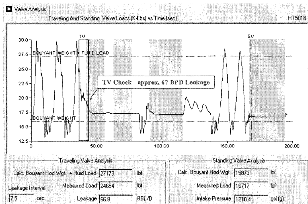
Figure 4 – Dynamometer Analysis, Valve Checks, Date 0911212002
