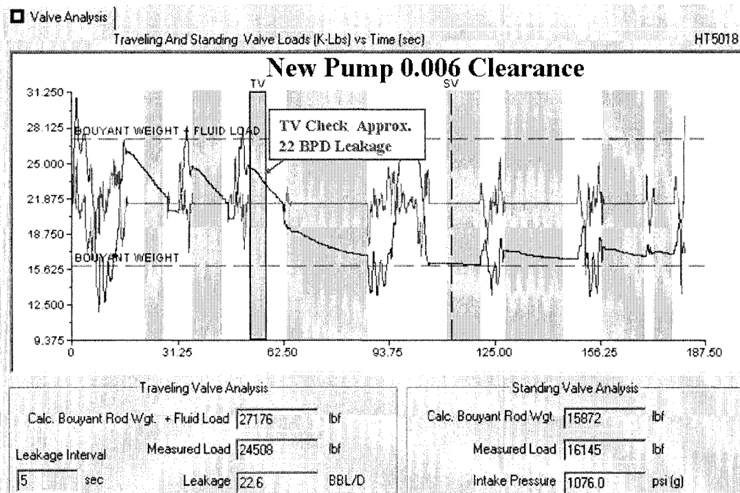
Figure 10 - Dynamometer Analysis, Valve Checks Fastest Strokes/Min, 10/22/2002
