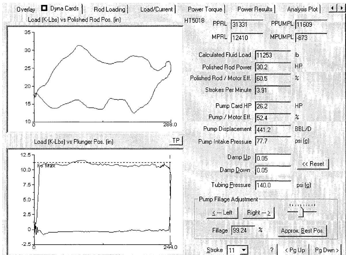
Figure 6 - Down-Hole Analysis, New Pump with 288 Stroke, Date 09/26/2002
