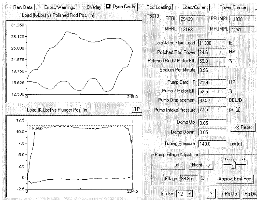
Figure 3 - Down-Hole Analysis, Leaky Pump with Shortened Stroke, Date 09/12/2002
