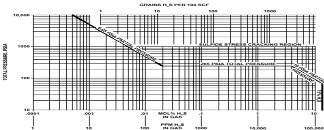
Figure1 - NACE MR0175 prior edition chart to determine potential for material to sulfide stress crack. (Ref. 2)
