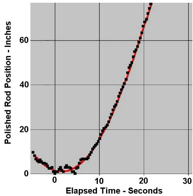
Figure 3 – Polished Rod Position from Inclinator Requires Smoothing of Error
