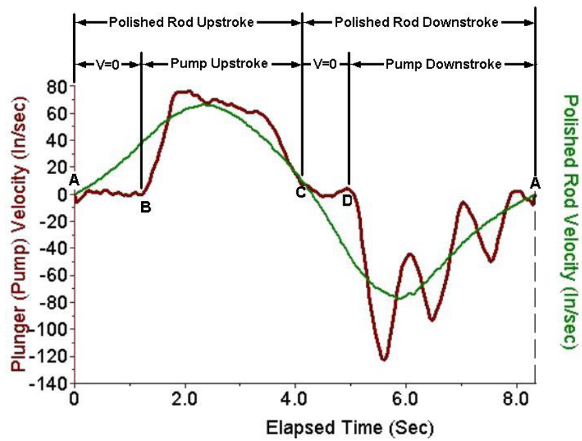
Figure 5 – Polished Rod and Plunger Velocity Versus Elapsed Time for Anchored Tubing
