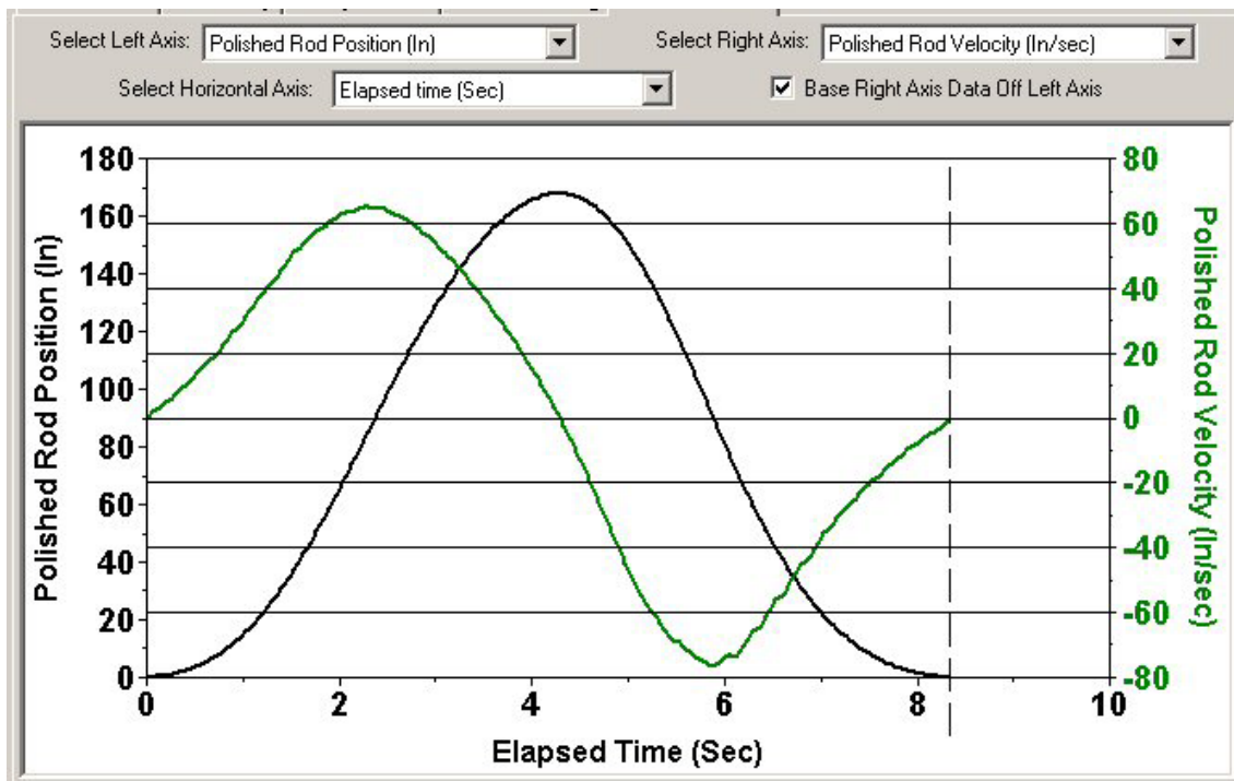
Figure 2 – Polished Rod Position is the Integration of Velocity with Respect to Time
