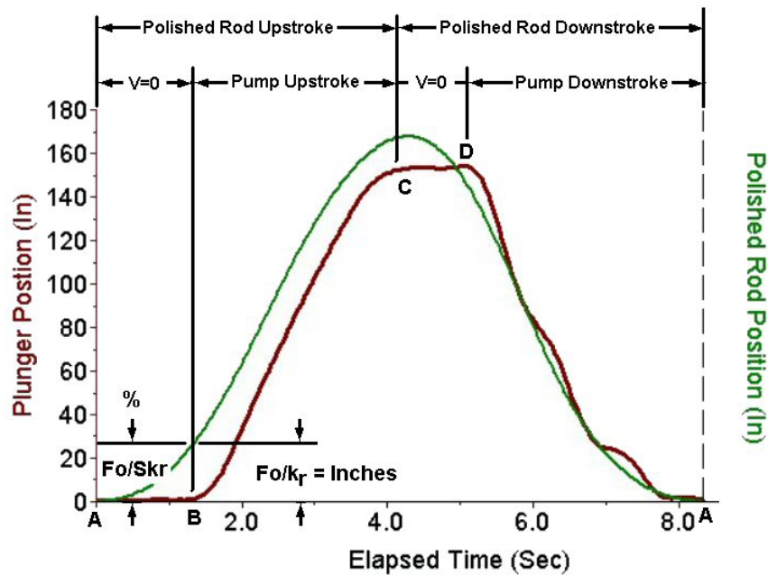
Figure 4 – Polished Rod and Plunger Position Versus Elapsed Time for Anchored Tubing
