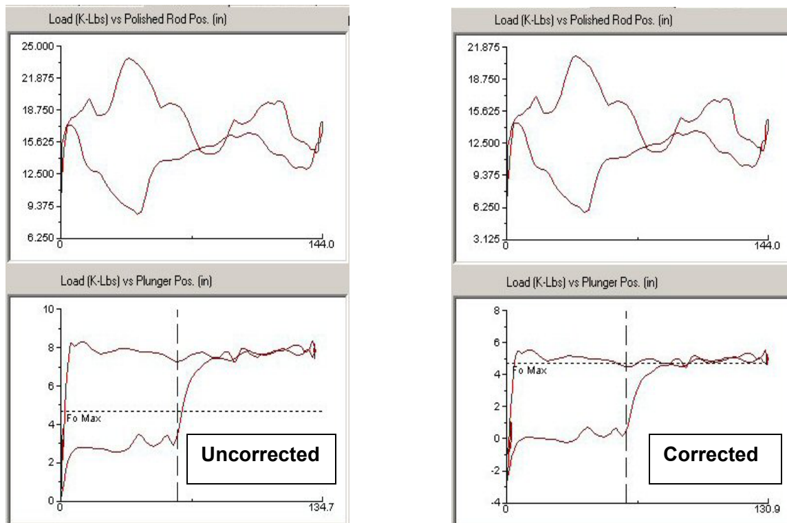
Figure 8 – Surface PRT Dynamometer Adjusted for Load Offset due to Tagging on the Down Stroke
