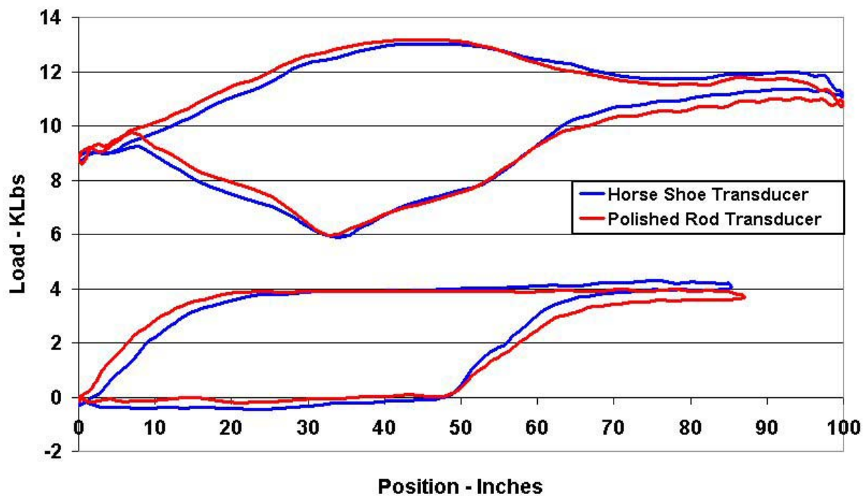
Figure 9 – Comparison of Polished Rod and Pump Dynamometer Cards for PRT and Load Cells
