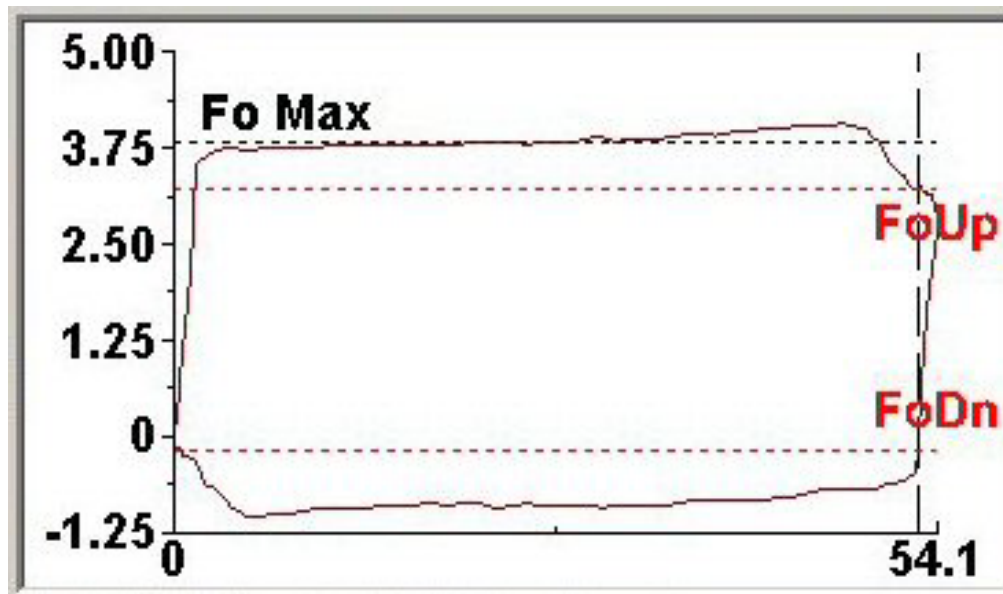
Figure 7 – Pump Card with Unaccounted Friction from Paraffin
