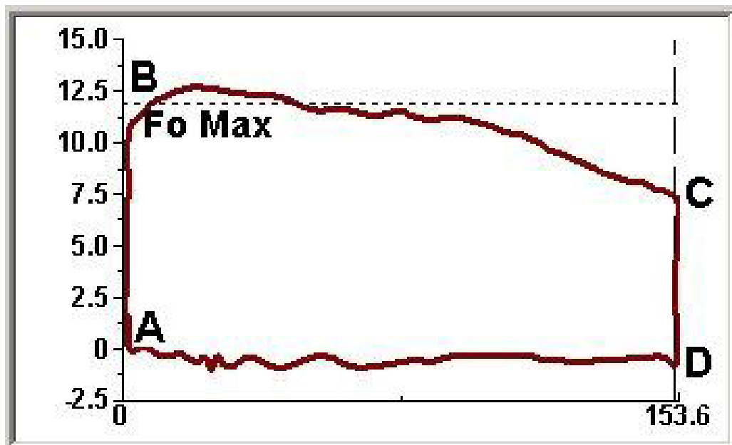
Figure 6 – Example Pump Card w/ Load (k-lbs) and Position (inches)
