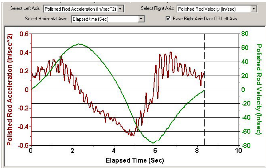
Figure 1 – Polished Rod Velocity is the Integration of Acceleration with Respect to Time
