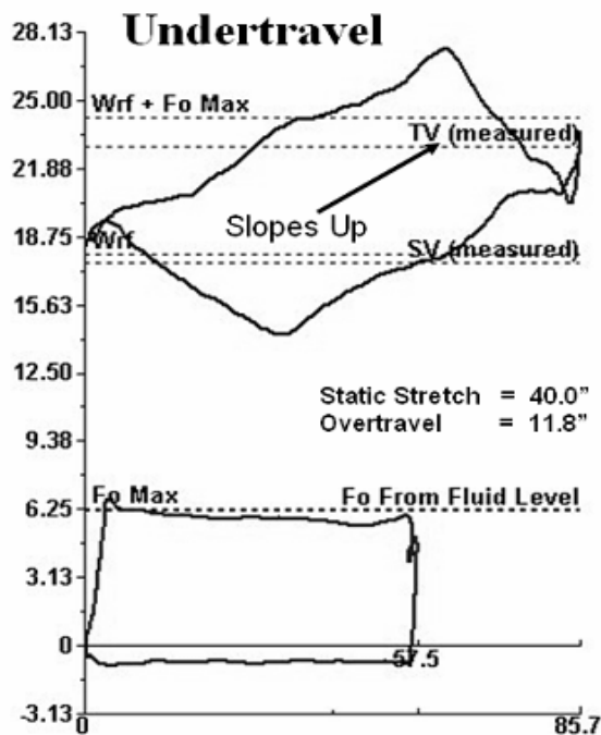
Figure 10 - Undertravel surface and pump cards and loads with discussion of undertravel.
