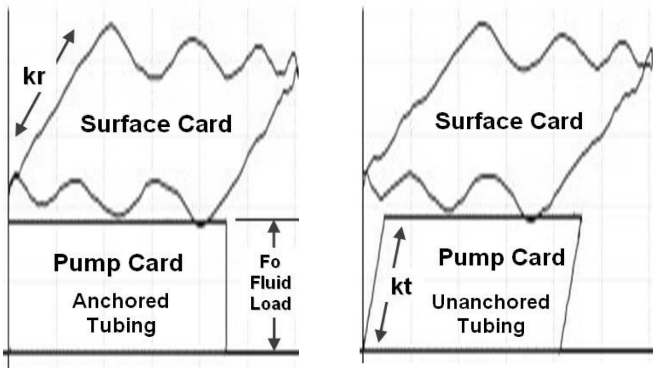
Figure 3 - Example of Predicted Surface Dynamometer from Pump Conditions for Anchored and Unanchored Tubing.
