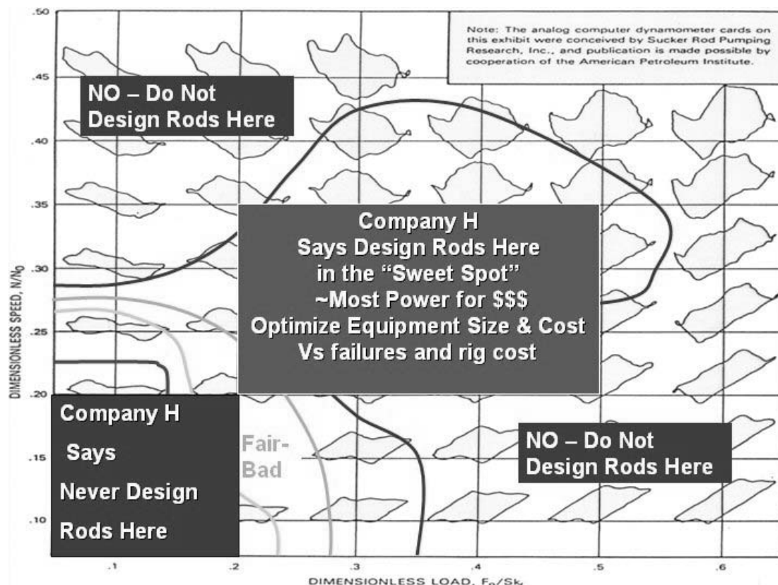
Figure 12 - Comparison of two different companies recommended sucker rod non-dimensional operating parameter Company H; bound by 0.2 to 0.35 N/N_0 and 0.2 to 0.5 F_o/S_{kr}
