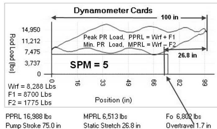
Figure 6 - Example well surface and pump cards and loads with N = 5 spm.
