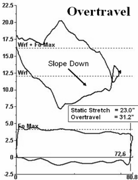
Figure 9 – Overtravel surface and pump cards and loads with discussion of overtravel.
