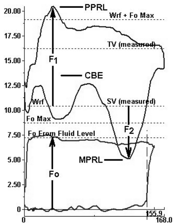
Figure 4 - Surface dynamometer (upper trace) and downhole (lower trace) pump card loads showing relationship of the major sucker rod string loads and some operating parameters.
