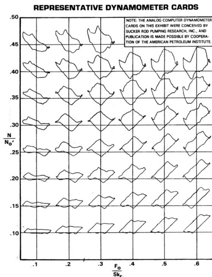
Figure 2 - Suite of analog dynamometer cards from API Bull 11L2 showing non-dimensional pumping parameters and the effect on card shape. Ref. 5.
