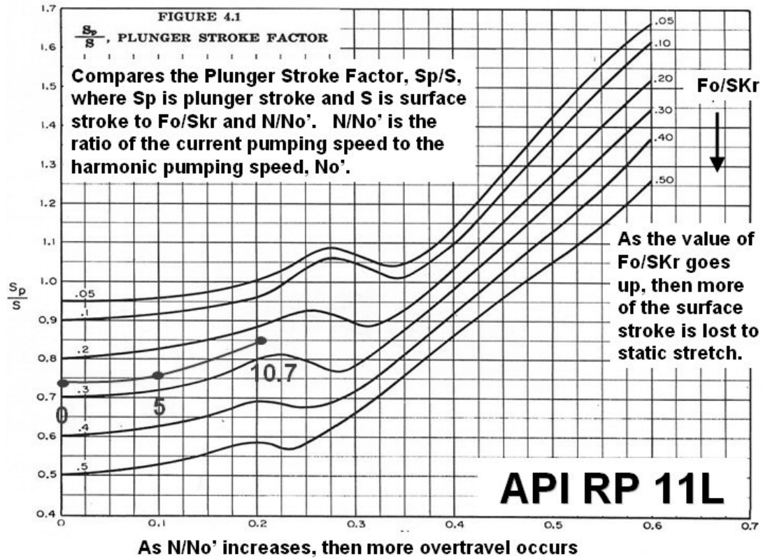
Figure 8 - API RP 11L S_p/S vs. N/N_o'
