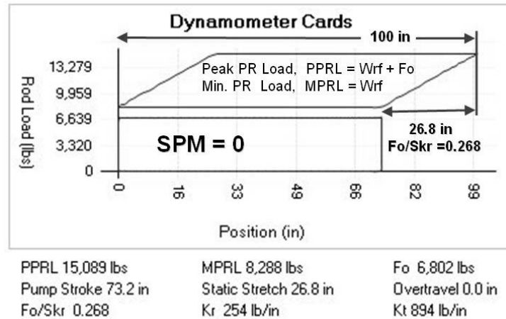
Figure 5 - Example well surface and pump cards and loads with N = 0 spm
