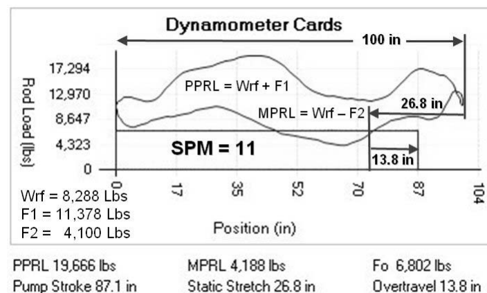
Figure 7 - Example well surface and pump cards and loads with N = 10.7 spm.
