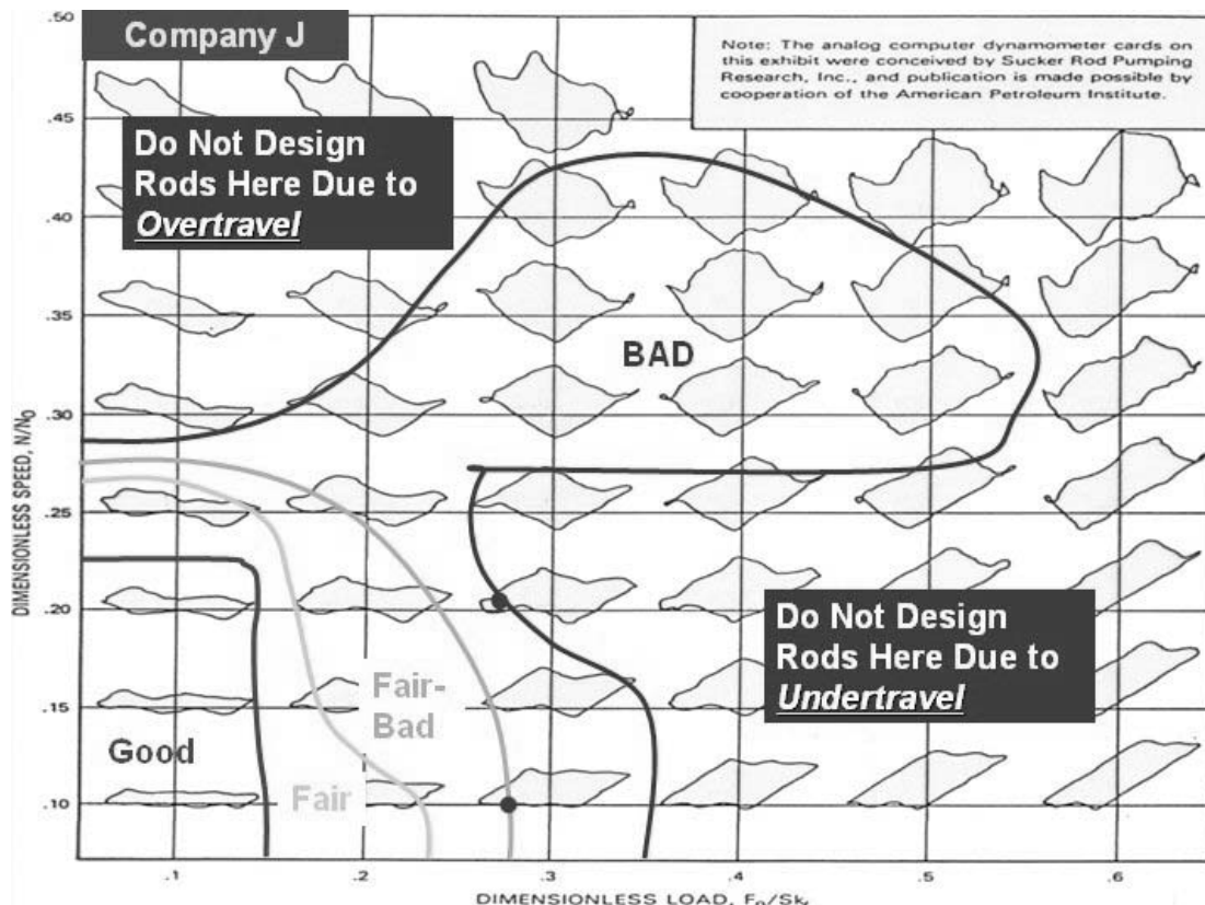
Figure 11 - Company J Rod String Design Limits bounds for N/No' and Fo/Skr .
