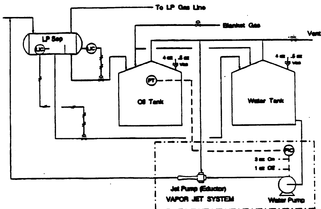
Figure 1 - Schematic - Vapor Jet Recovery System
