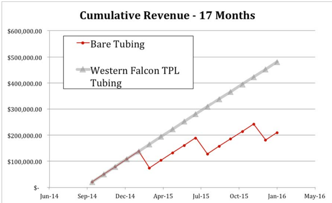
Figure 11 – Cumulative Single Well Revenue Averaging Approximately $187,000 of Incremental Gain Per Year over 17 Months, Before vs. After TPL Tubing Installation For Case Study Four
