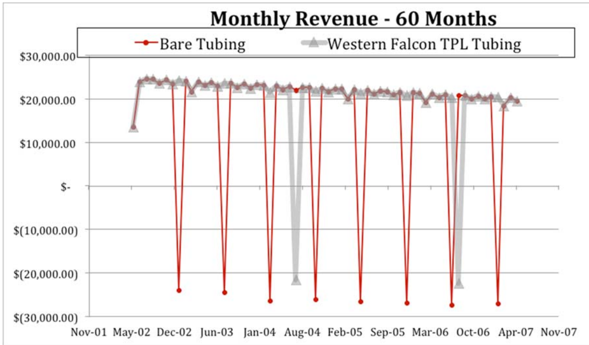
Figure 1 – Comparative Monthly Single Well Revenue Before and After Installation of TPL Tubing For Case Study One
