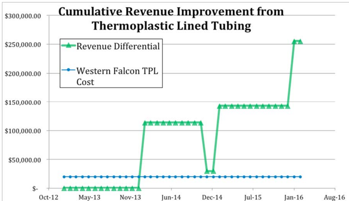
Figure 9 – Single Well Revenue Differential Over 39 Month Period After Installation of TPL Tubing Costing Less Than $20,000 For Case Study Three
