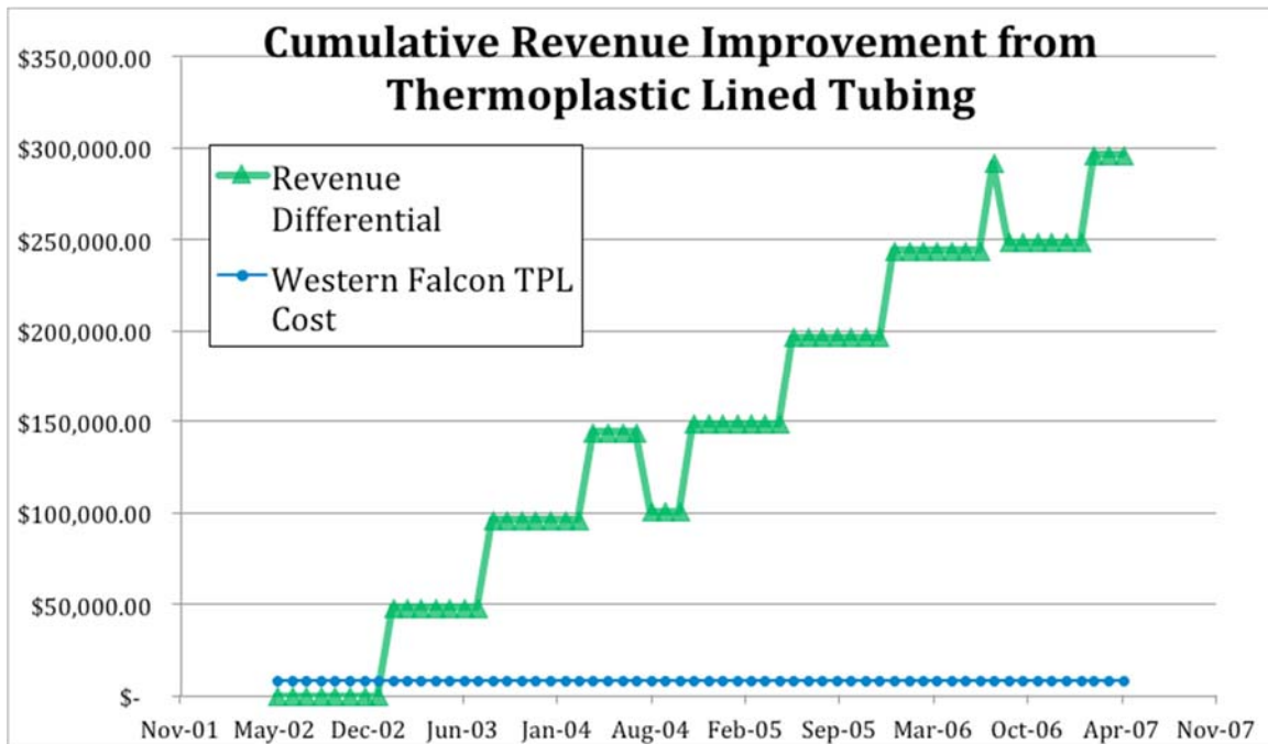
Figure 3 – Single Well Revenue Differential Over 5 Year Period After Installation of TPL Tubing Costing Less Than $9,000 For Case Study One
