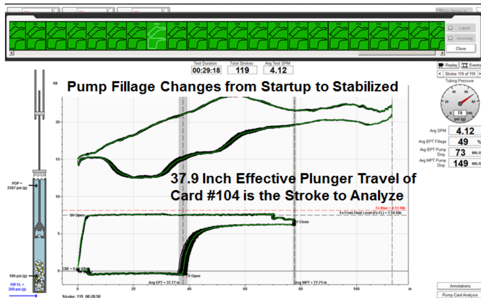
Figure 6 – Selection of Representative Stroke 104 for Analysis from Pump Card Overlay
