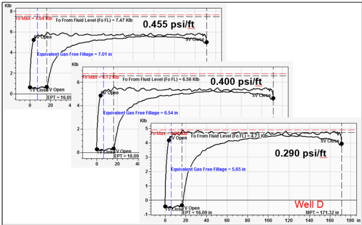
Figure 14 – Effects of Manually Adjusting Tubing Fluid Gradient on Well D
