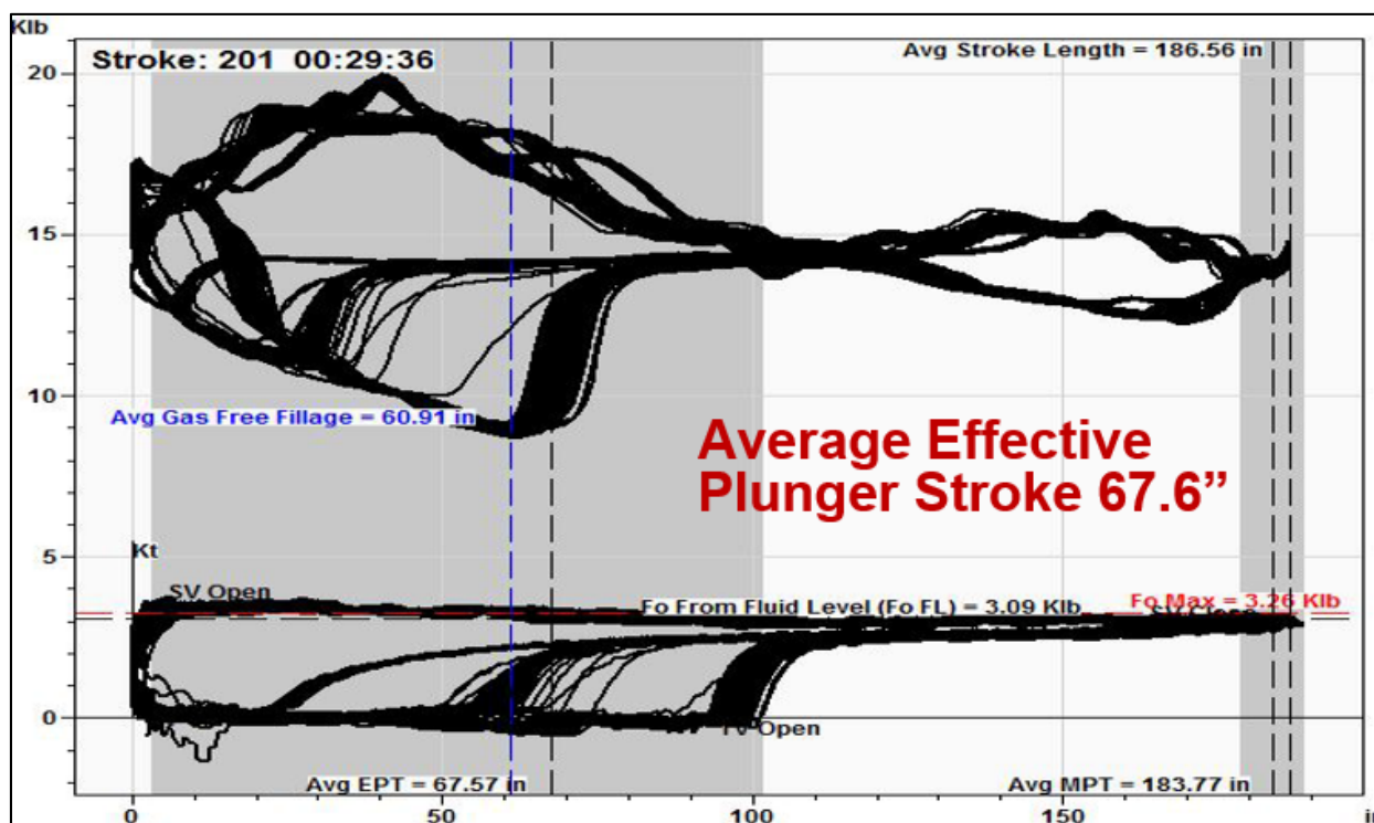
Figure 11 – Pump Card Overlay Displaying Changes in Pump Filling on Well C
