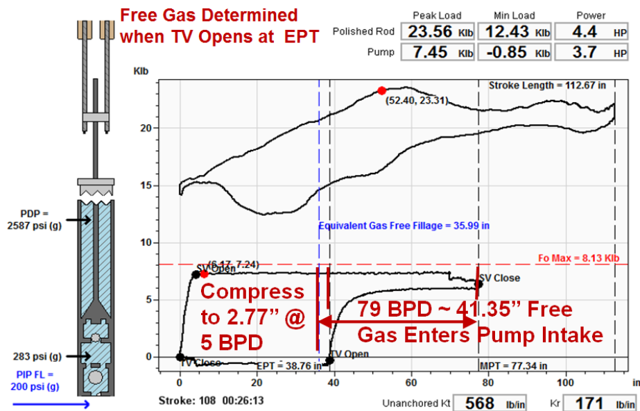
Figure 3 – Compressed Gas Volume in the Pump Chamber
