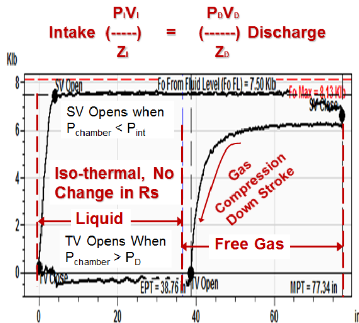
Figure 4 – Z-Factor Calculations
