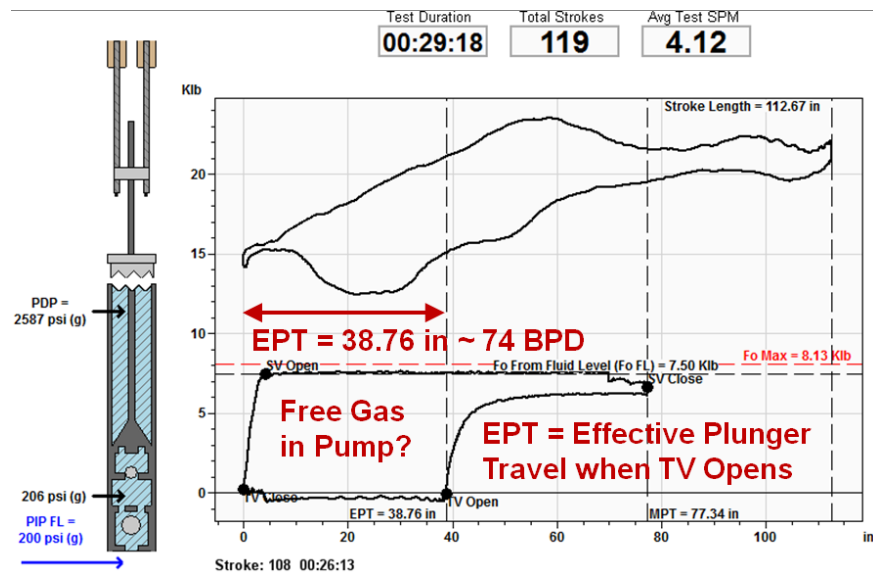
Figure 1 – Example of Difference in Pump Displacement Calculation and Surface Measurements
