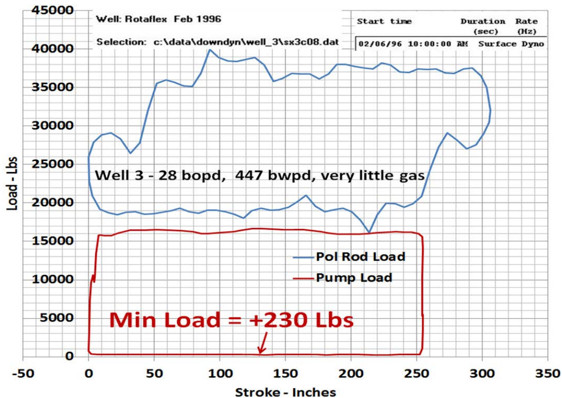
Figure 9 – Effective Load Surface and Pump Card Loads for Well_3
