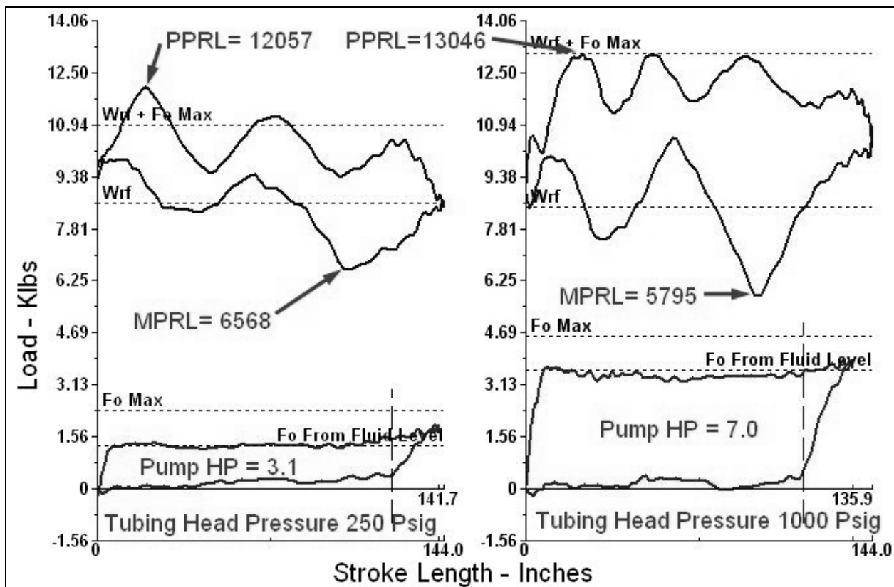
Figure 3 – Compare Dynamometer Cards of 250 to 1000 psig of Backpressure
