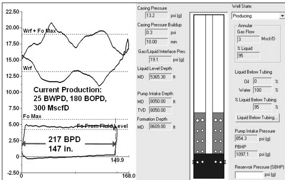
Figure 4 – Initial Fluid Level and Dynamometer Data Collected at Initiation of Sucker Rod Lift
