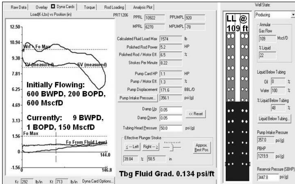
Figure 1 – Well Flowing off Tubing and Casing with Fluid Level at/near Surface: Poor Pump Action & Low Production Rate
