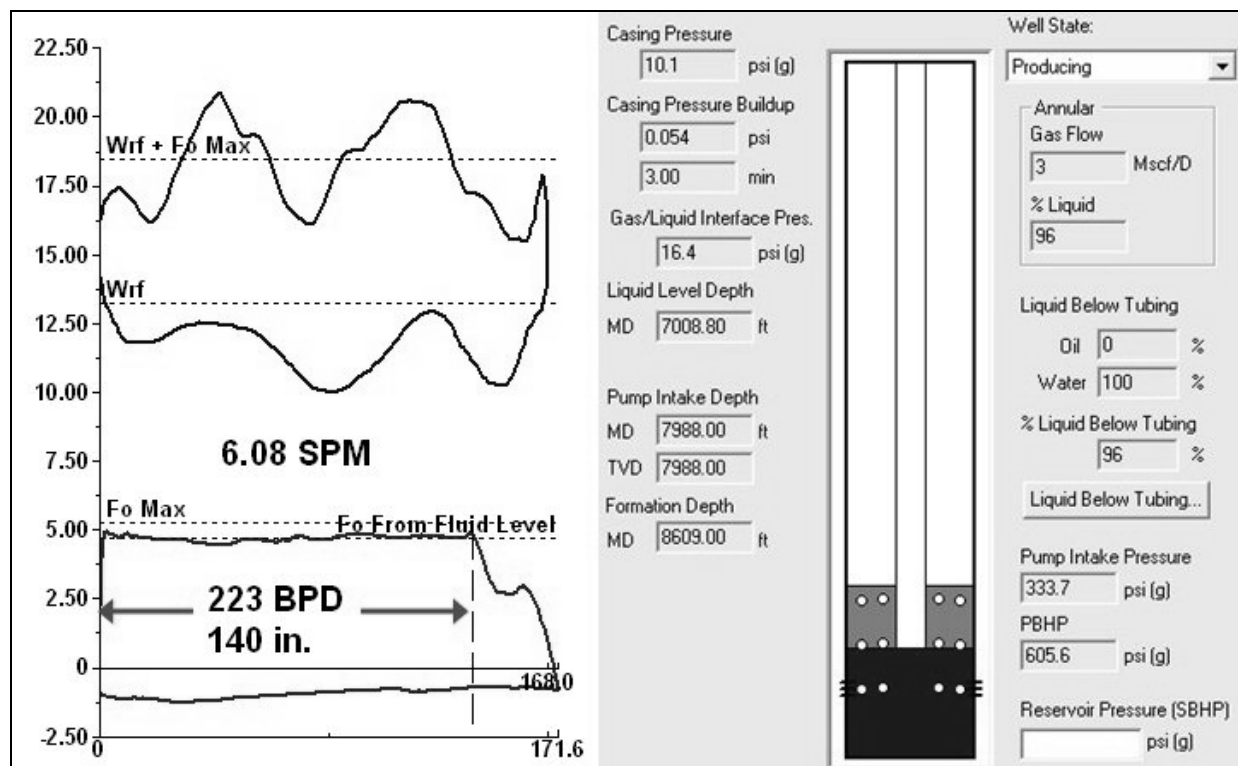
Figure 7 – Dynamometer and fluid Level Data after Variable Slippage Pump and Improved Downhole Gas Separator Installed
