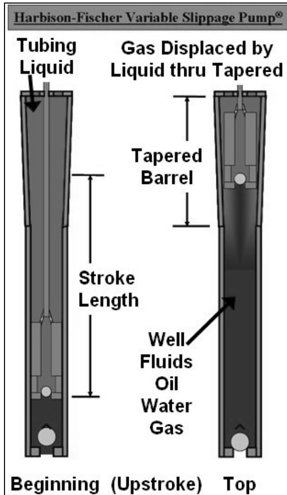
Figure 9 – Harbin-Fisher Variable Slippage Pump
