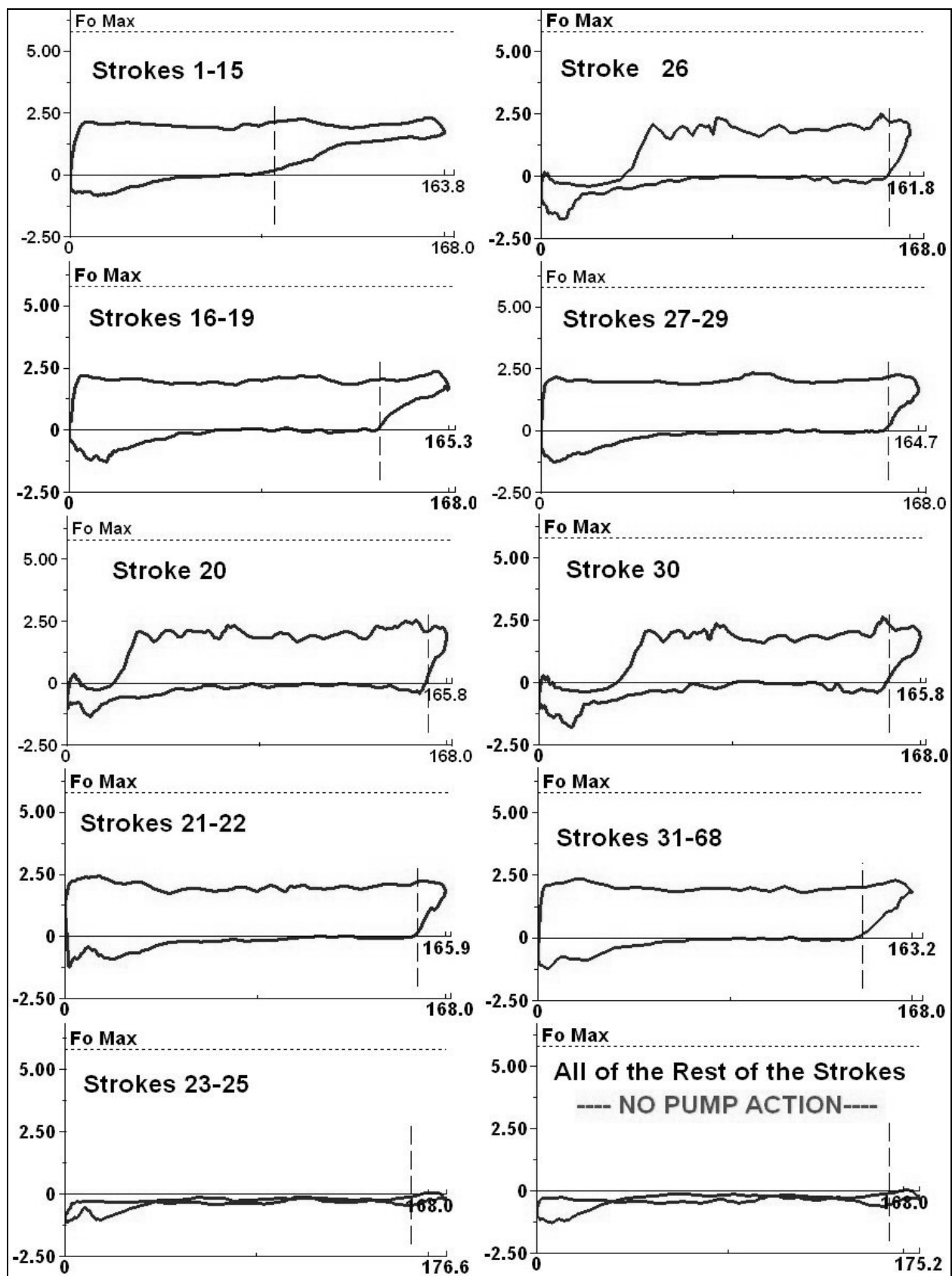
Figure 6 – Sequence of Pump Cards Showing Unstable Pump Action
