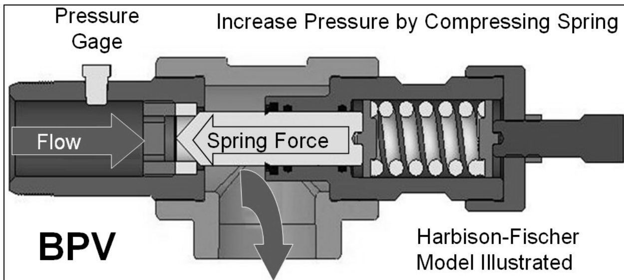
Figure 2 – Backpressure Regulating Valve
