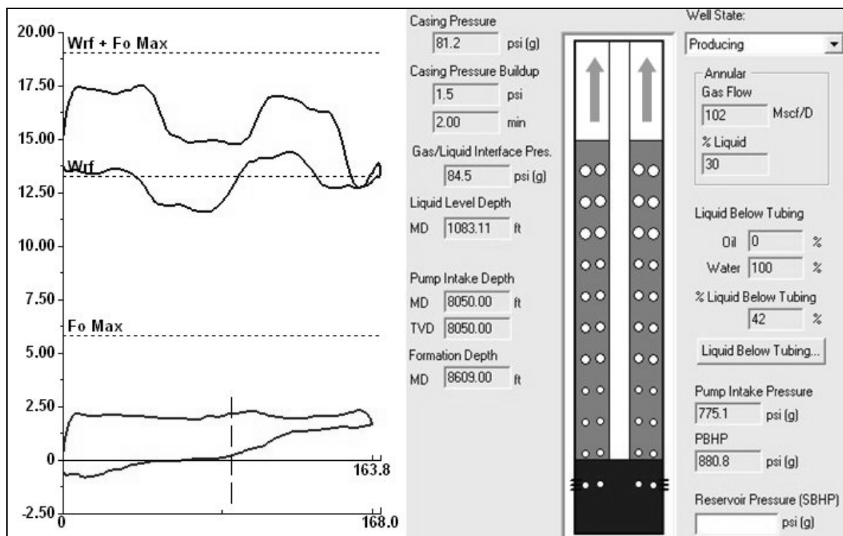
Figure 5 –Follow-up Fluid Level and Dynamometer Data Collection 5 Days After Initiation of Sucker Rod Pumping
