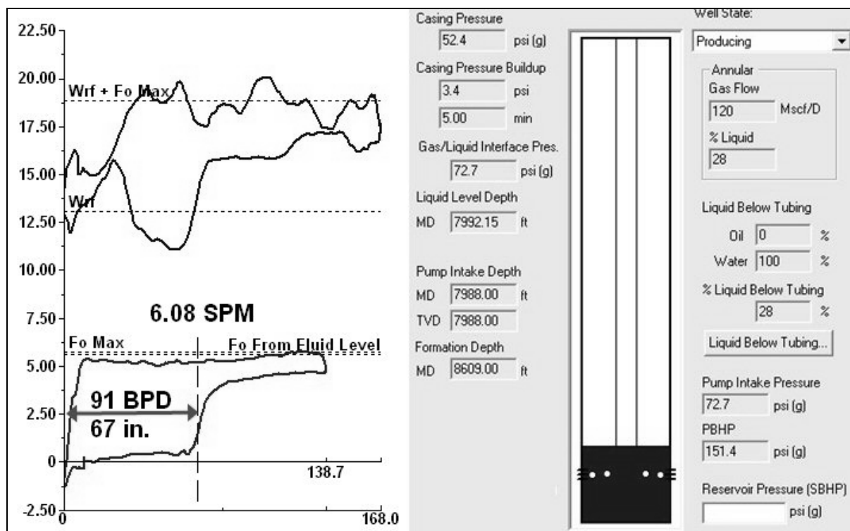
Figure 8 – Dynamometer and Fluid Level Data Seven Months Later
