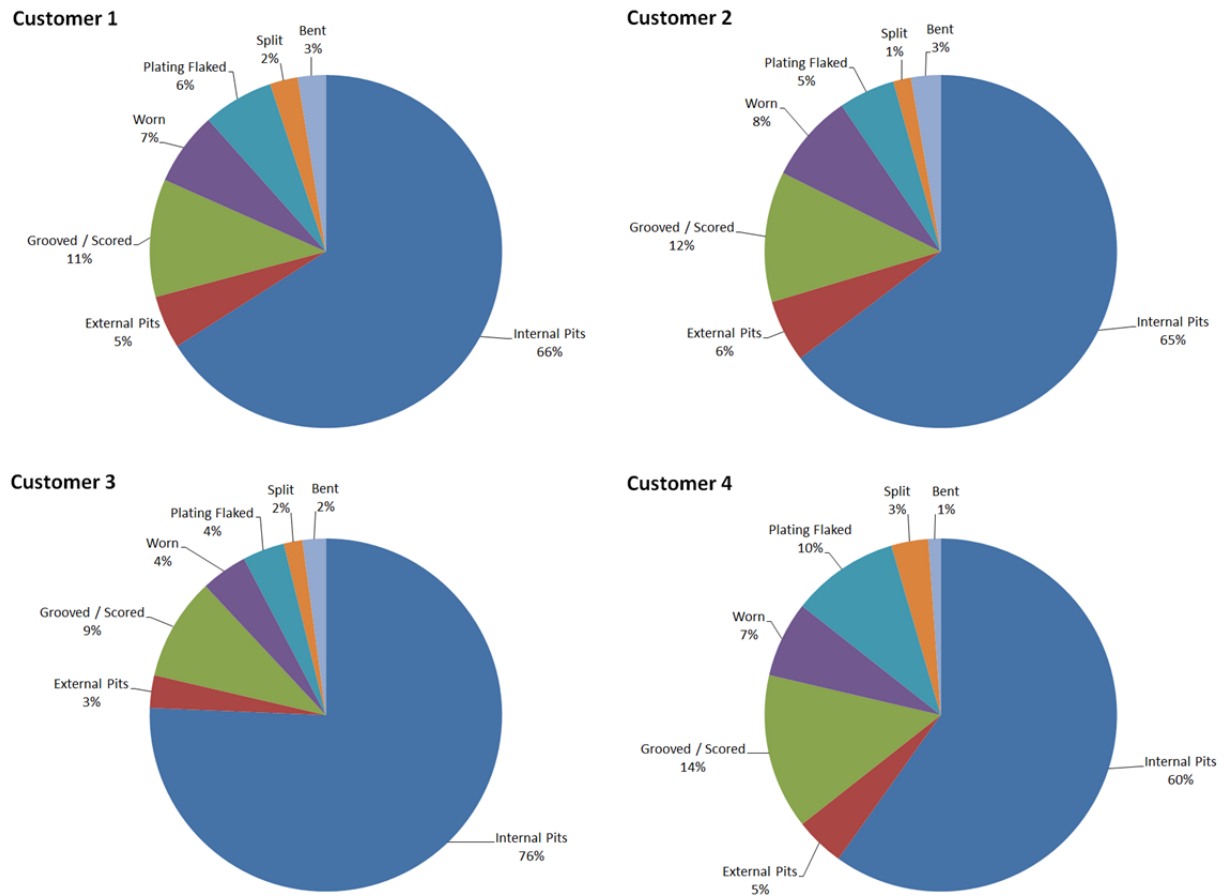
Figure 2 - Failures modes in sucker rod barrels for 4 major companies at Permian Basin
