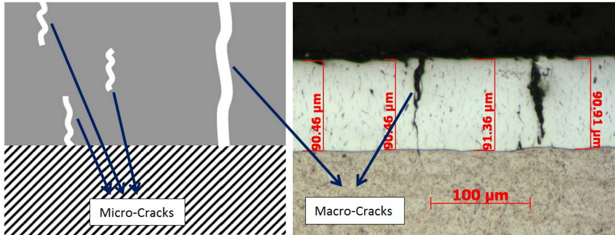
Figure 1 - Micro and macro-cracks in Chrome plating.
