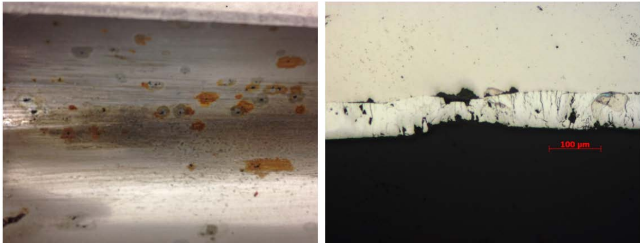
Figure 3 - Random, shallow corrosion pits on the barrel surface.
